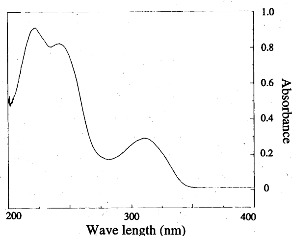
Fig. 2. UV spectrum of cystothiazole A ( 2.39 \times 10^{-5} M in MeOH).
